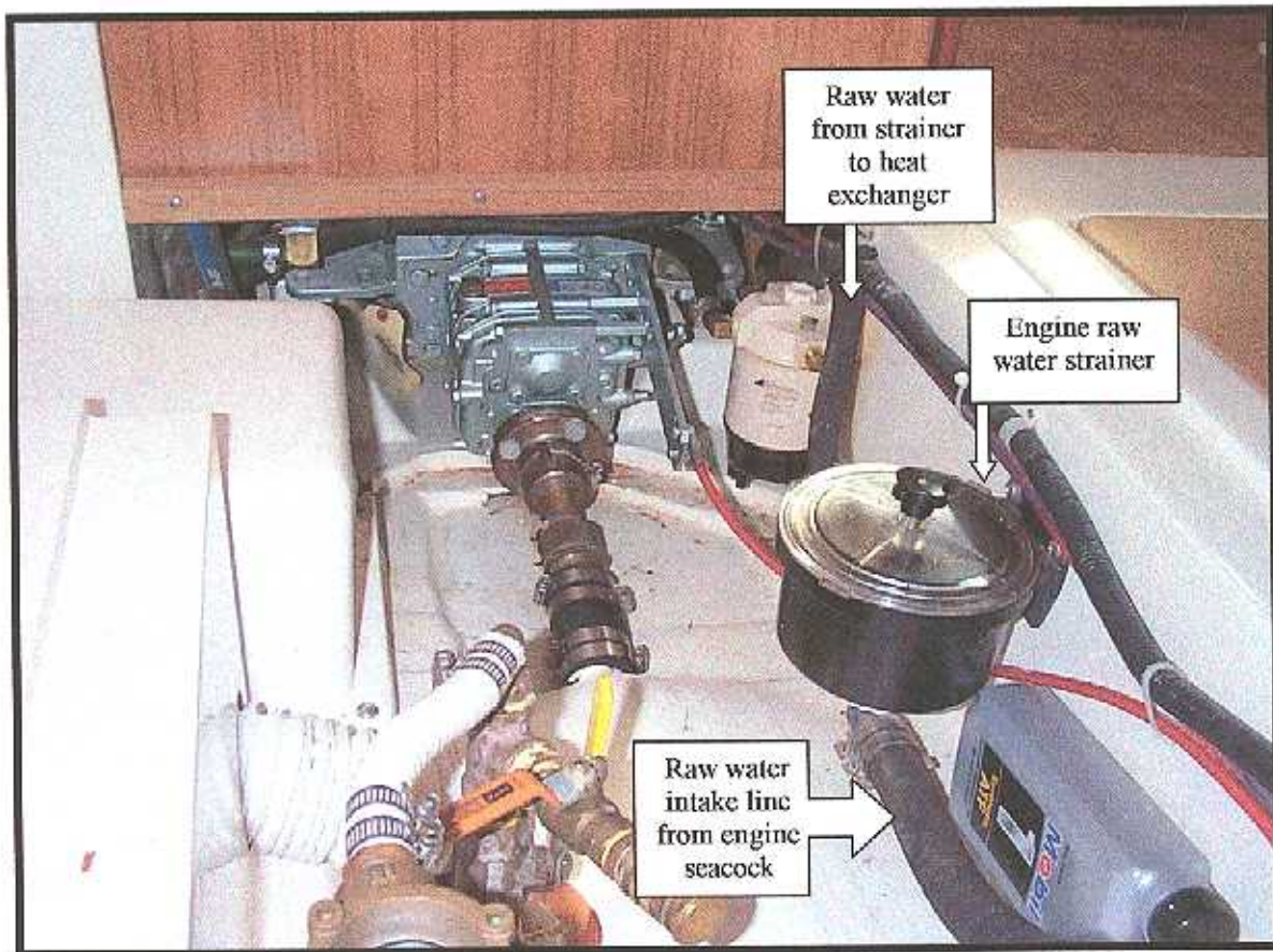
Figure 2.2 Raw water strainer. Aft Cabin - Picture taken from stern looking toward the engine
