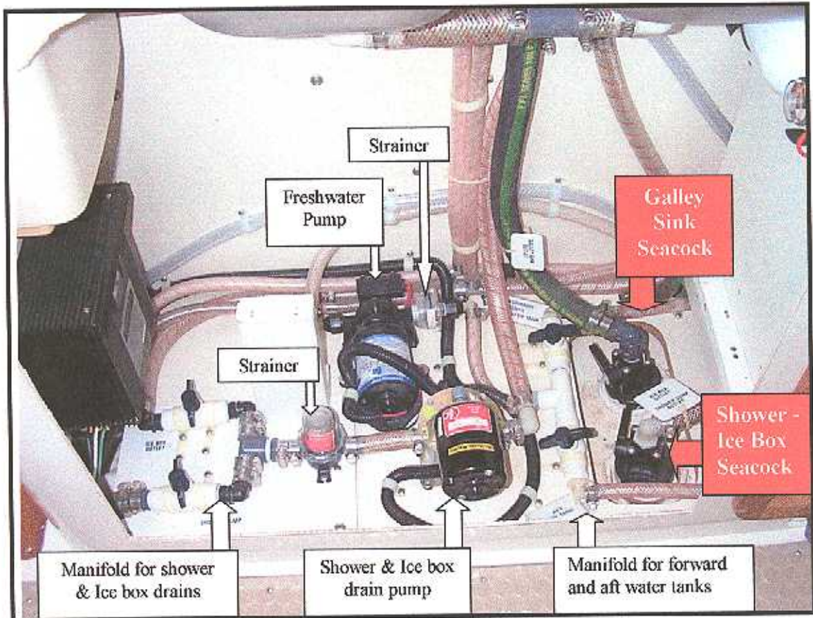
Figure 2.8 Potable water system – equipment mounted in the cabinet under the galley sink (photo taken from aft cabin looking forward – cabinet doors and horizontal shelf removed for picture)
