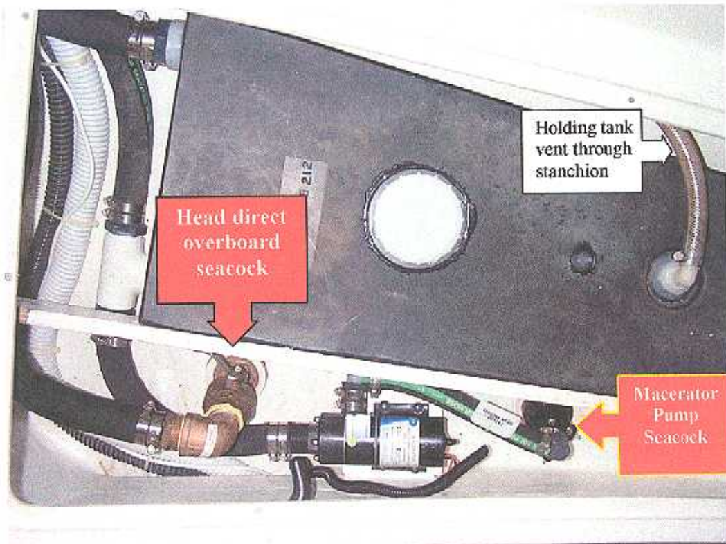
Figure 2.8 Holding tank, Head direct overboard discharge, Macerator pump and seacock.
