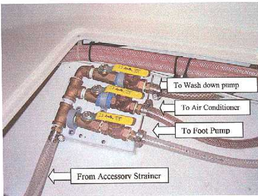
Fig 2.5 Accessory seawater manifold
