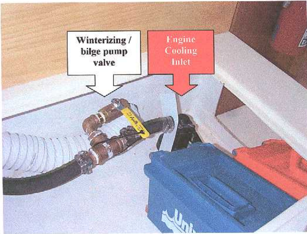
Fig 2.1 Engine Cooling inlet and winterizing/bilge pump valve
