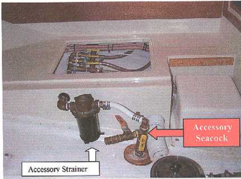
Fig 2.4 Accessory seawater intake system
